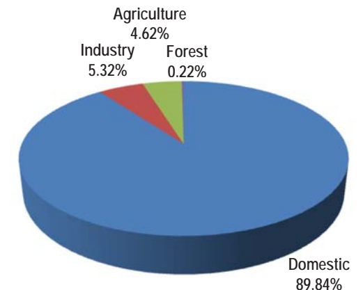
Figure 8. Total Nitrogen Loading of 58 Sub-basins (79,621 MT/yr) for 2008.
