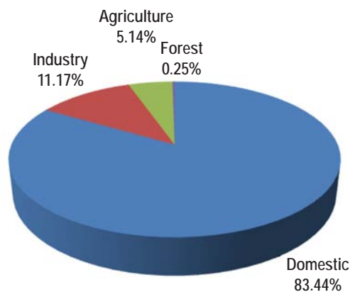
Figure 6. BOD Loading of 58 Sub-basins (232,764 MT/yr) for 2008.
