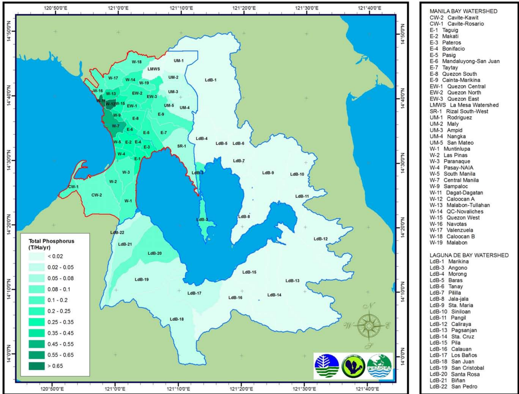
Figure 16. Map of Total Phosphorus Loading per Area in 58 Sub-basins for 2020.
